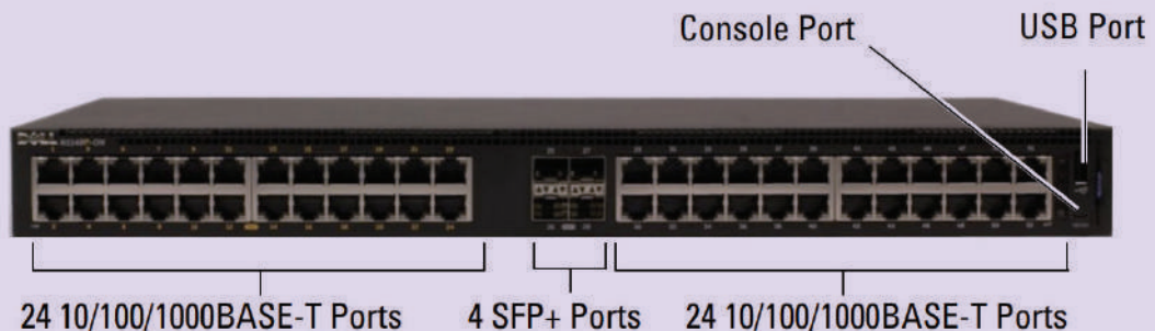
Dell EMC Networking N1148P-ON Switch (Front Panel)
