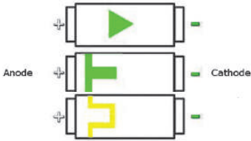
Surface Mount LED Polarity Indicators Underside of an SMD LED
